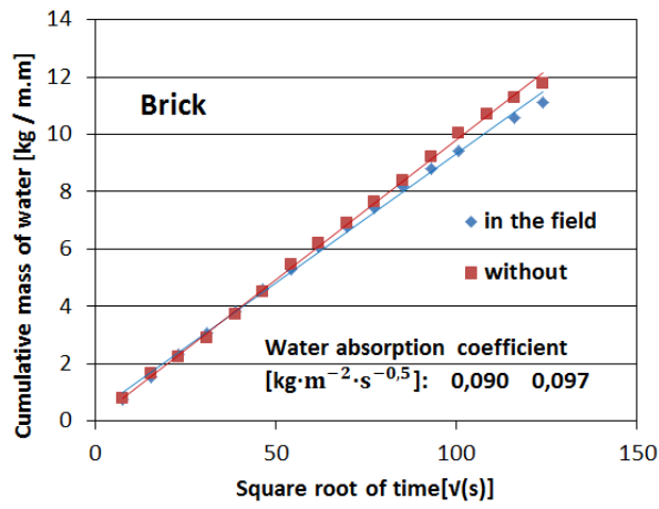
Fig. 7. Sorptivity plot for historic brick.
